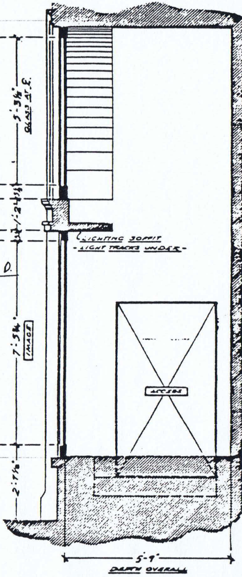
SECTION
